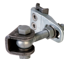
detail 180° scharnier
